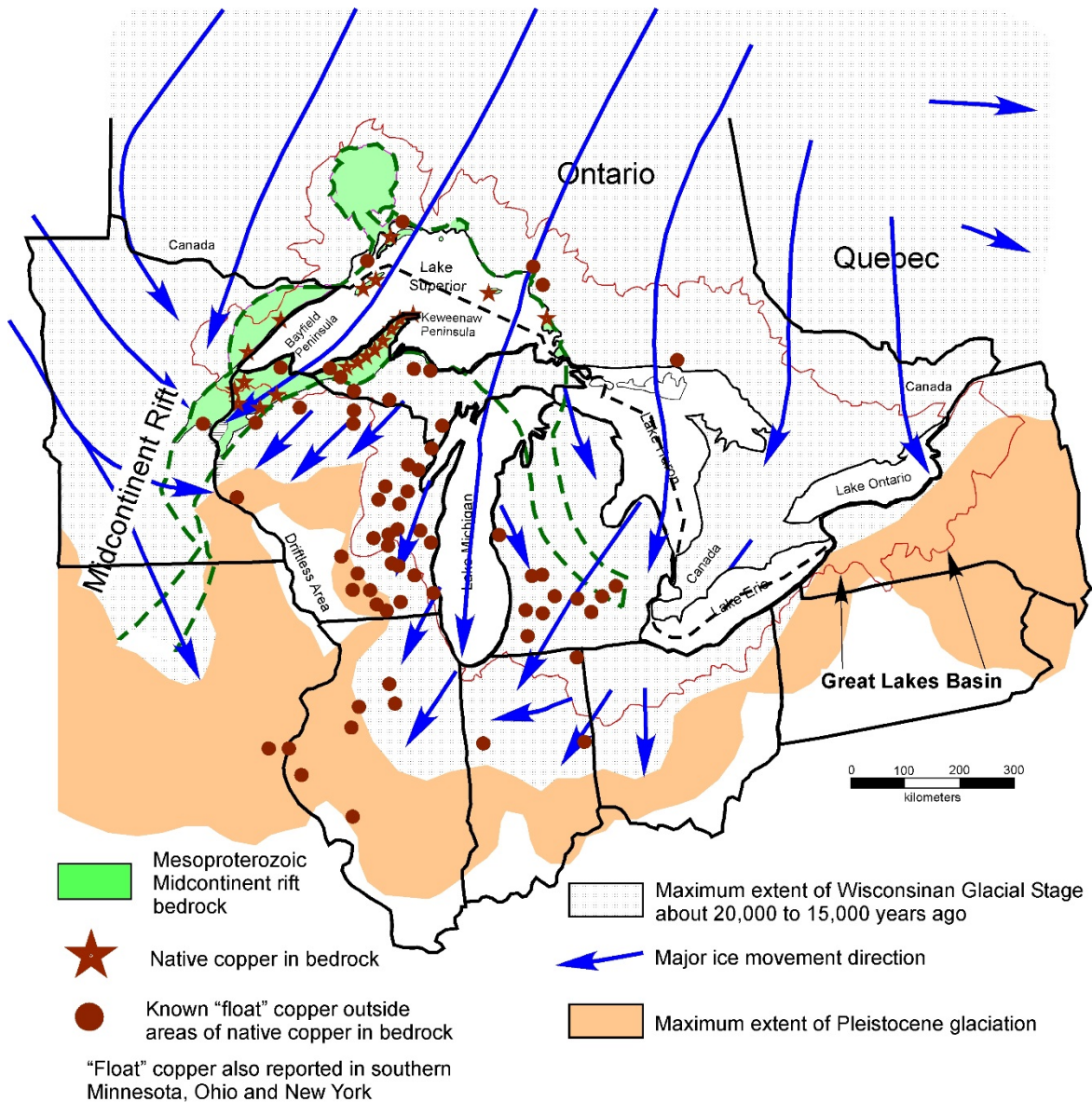
Figure 1: Map showing location of the native copper deposits of the Keweenaw Peninsula and the extent of float copper transported south by movement of glacial ice. Location of float copper from (4, 5 cited in 6, and 6)
